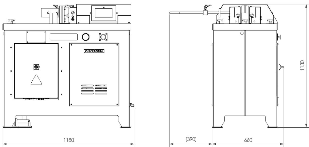
Figure 1. External Dimensions of the Horizontal Press Brake
