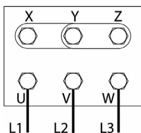
Figure 9. Wye configuration for 400 V voltage (pre-set)
