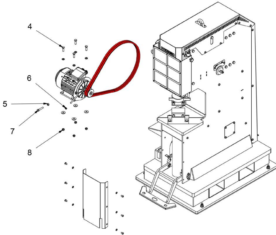
Figure 7. Main drive belts
