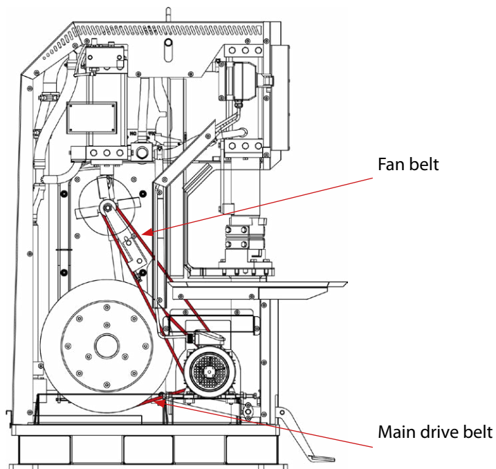
Figure 5. Transmission belts
