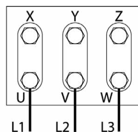
Figure 10. Delta configuration for 220 V voltage
