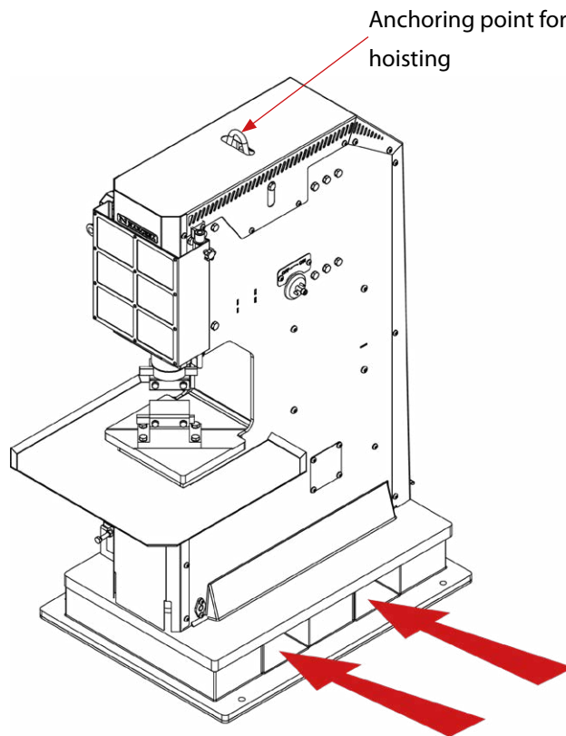
Figure 4. Moving the machine
