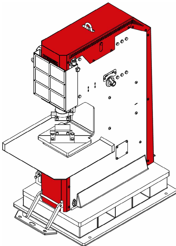
Figure 3. Power Hammer protective guards
