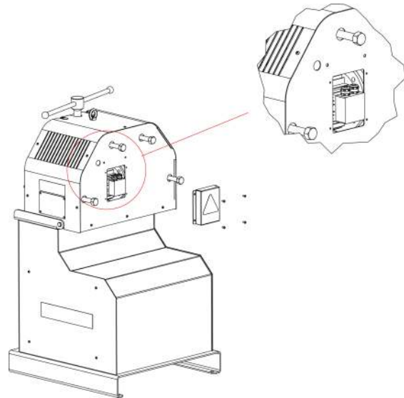
Figure 7. Change of engine connections
