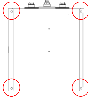
Figure 5. Anchor points of the machine
