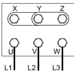
Star picture (preset) For tension 400V
