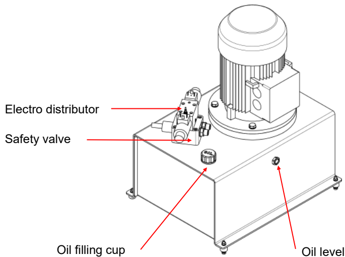
Picture 5. Identification of the Components of the hydraulic container
