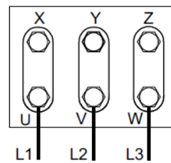
Picture 11. Triangle picture for tension 230V
