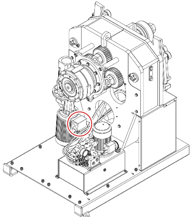
Figure 9. Engine connections
