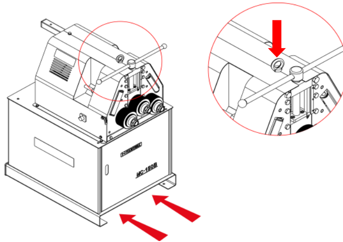
Figure 4. Transportation of the machine
