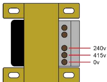
Figure 8. Change transformer primary connection
