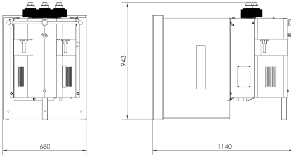
Figure 11. Machine dimensions with the base-plate in a horizontal position
