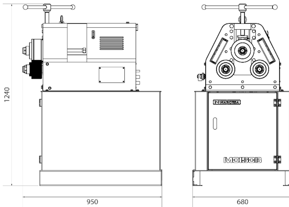
Figure 1. External dimensions of the MC150B bending machine
