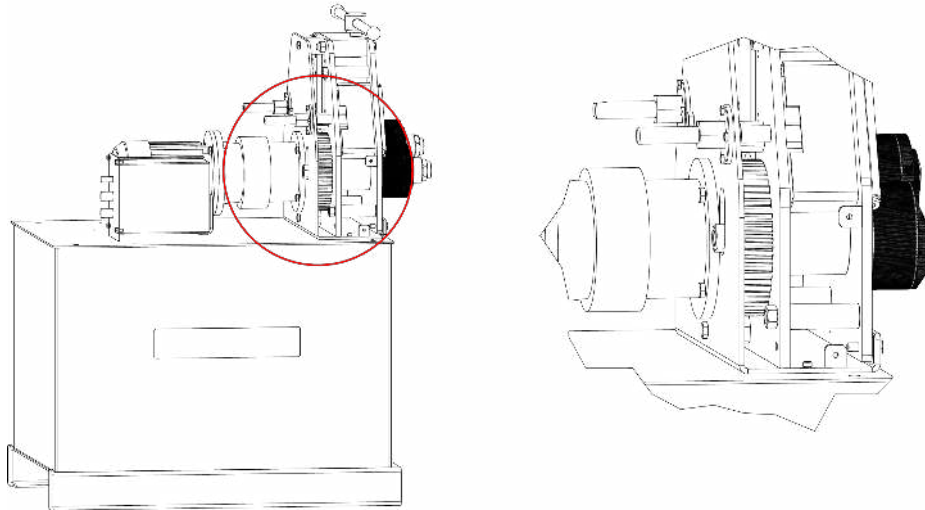
Figure 3. Mechanism protection guards
