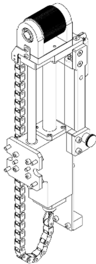
x1 Encoder set
