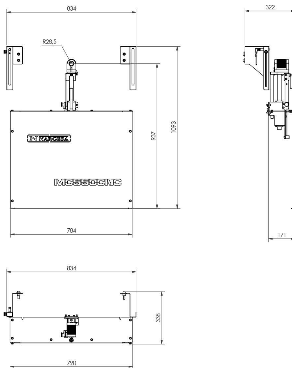
Figure 1. Outside dimensions of the MC550 bender
