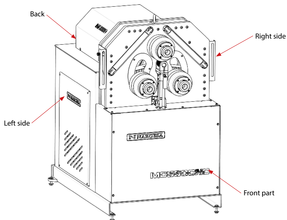
Figure 7. Detailed view of the machine areas.
