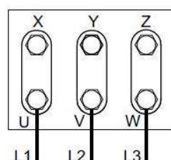
Triangular figure for 230V
