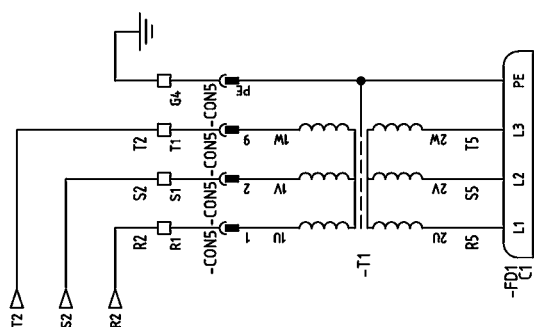
FD1 : BACK GAUGE MOTOR DRIVER CON5 : 16 PIN CONNECTOR
