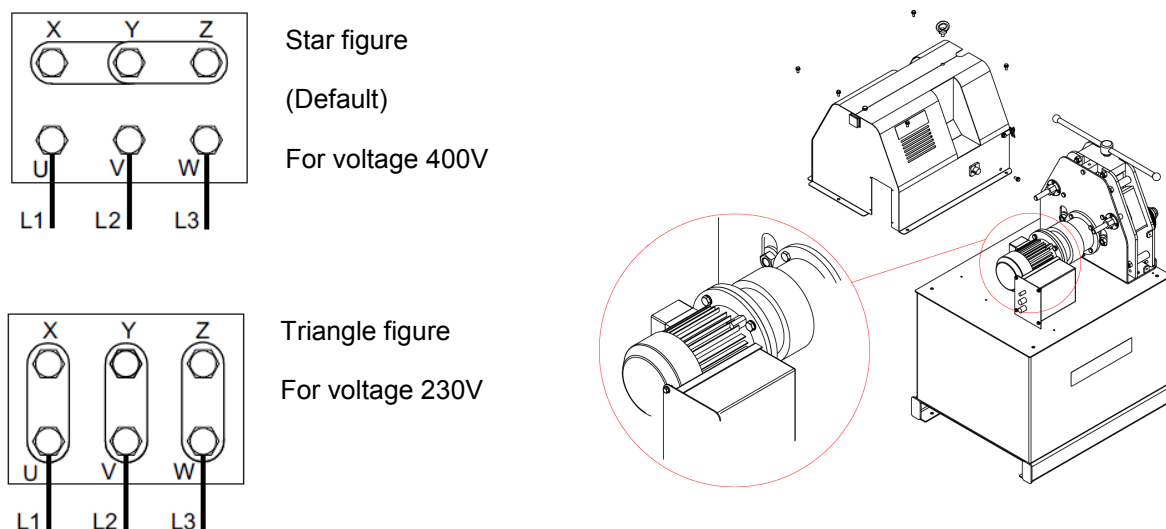
Figure 7. Change of engine connections
