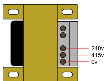
Figure 8. Change transformer primary connection
