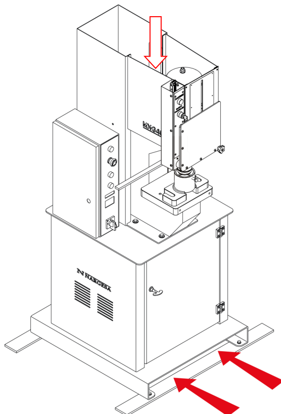
Figure 4. Transport de la machine
